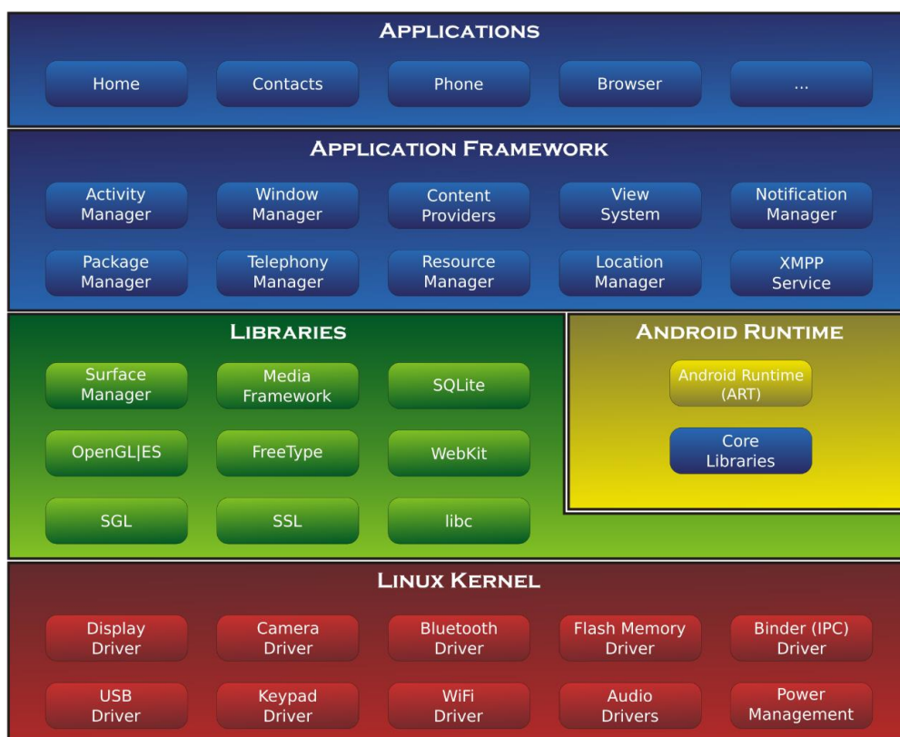
Figure 2. Diagrammatic Views of Android Architectures[19].
